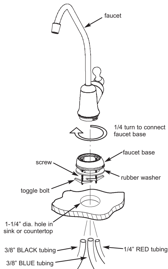
FIGURE 3 - FAUCET INSTALLATION
